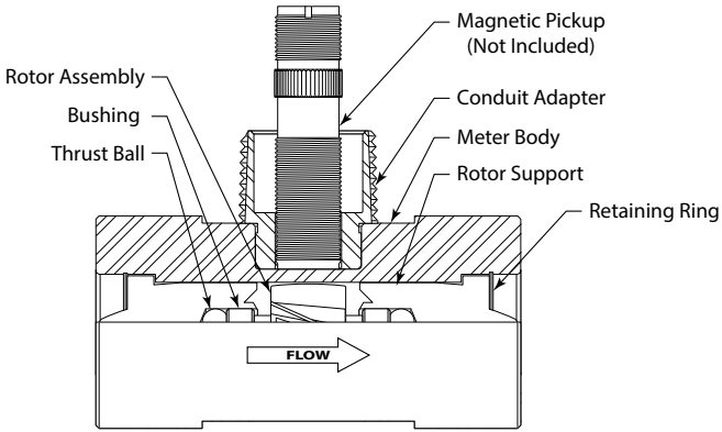
Figure 5: Typical cross-section of models BP131C-038...BP131C-100
