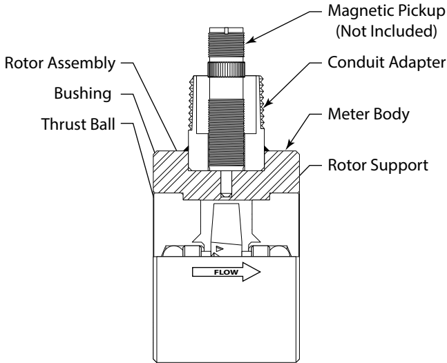
Figure 6: Typical cross-section of models BP132C-050...BP139C-900
