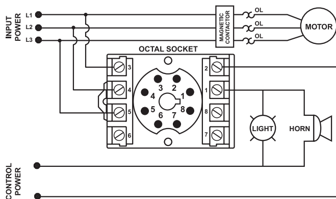
TYPICAL WIRING DIAGRAM FOR MODEL 201A-AU WITH ALARM CONTROL
