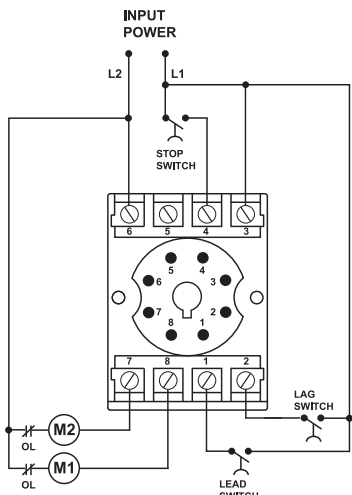
TYPICAL WIRING DIAGRAM FOR ALT-xxx-3-SW
