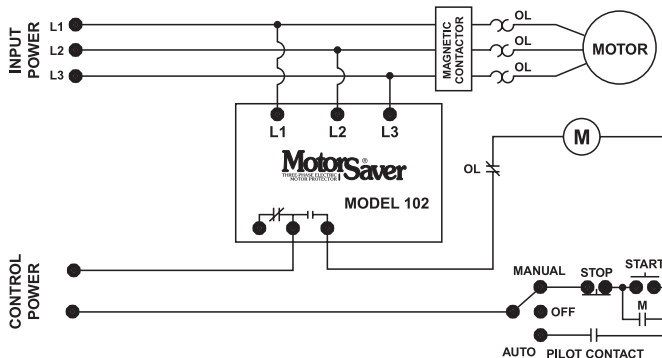
TYPICAL WIRING DIAGRAM FOR MODEL 102 WITH MOTOR CONTROL
