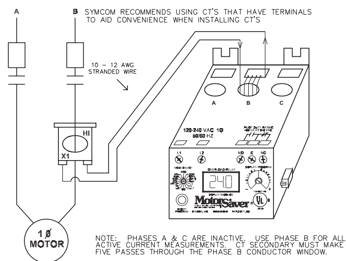
TYPICAL WIRING DIAGRAM FOR MODEL 77C WITH EXTERNAL CT
